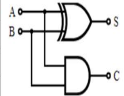
Half-Adder Schematic
